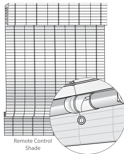
Motor Tube and Spindle
